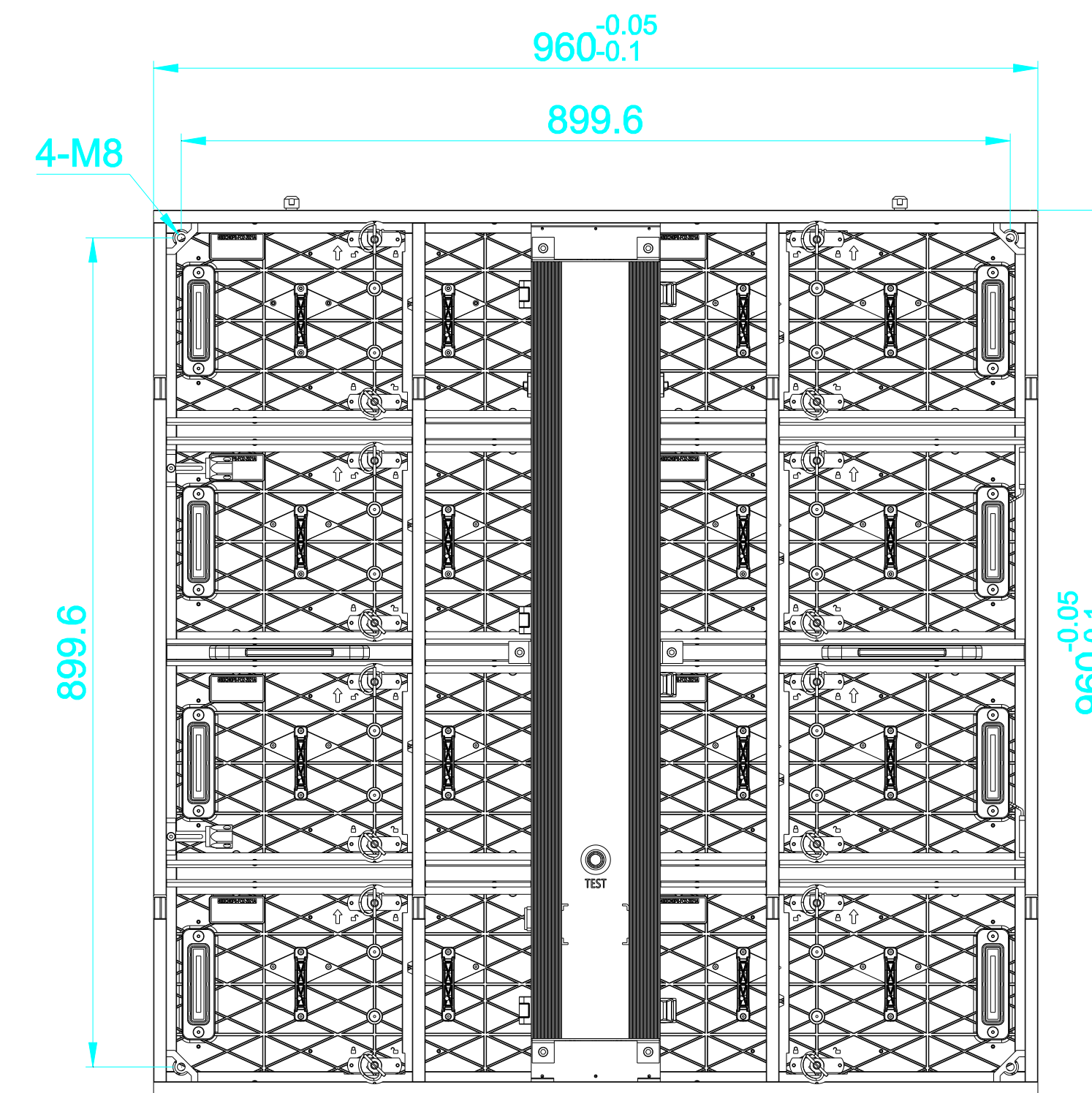
Rear view
