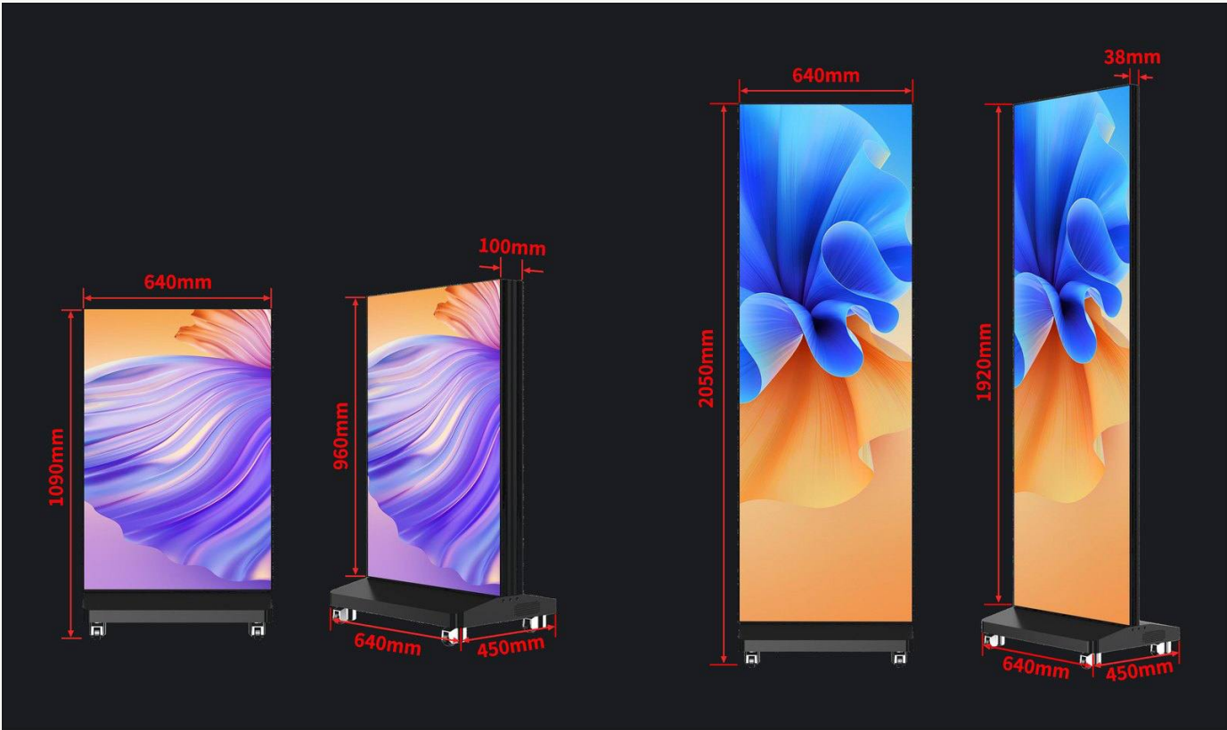
Left: folded, 640 mm wide, 1,090 mm high, 100 mm thick. Right: open, 2,050 mm high on the base, 38 mm cabinet. Manufacturer's drawing.
